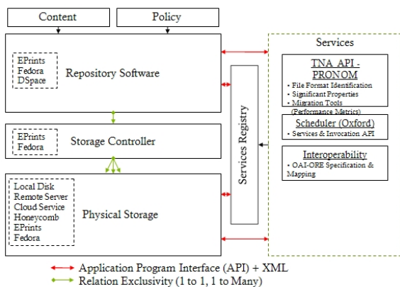
Figure 4: Storage-services based model of Preserv 2 development programme
